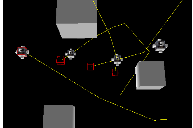
Figure 1: Motion Planning for 4 free-floating robots in a 3D space environment. Yellow lines denote robot trajectories that end at goal locations denoted by red cube lattices. The large gray cubes denote obstacles.
