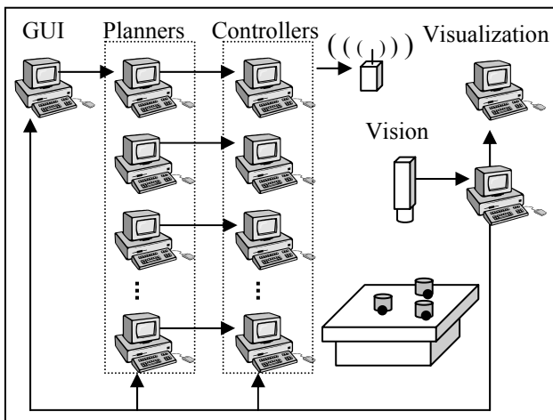
Figure 4: Network architecture of MARS test-platform
