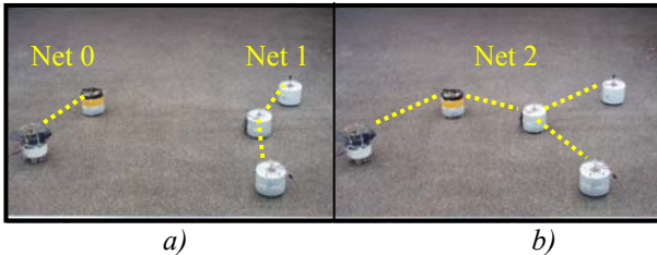
Figure 2: Example with 5 robots. Dashed lines between robots depict communication links. In a) the robots form two distinct networks Net0 and Net1. In b), two robots have moved, and the two networks in a) have merged into Net2.
