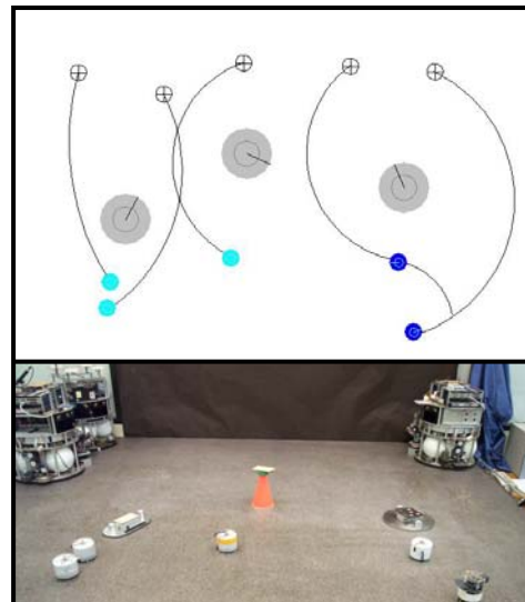
Figure 5: Example experiment on the MARS test-platform involving 5 robots and 3 obstacles.
