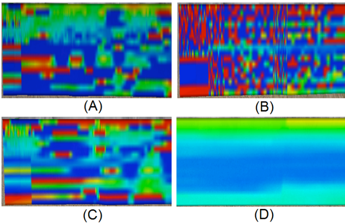
Figure 5: A comparison of radial basis function interpolation with different basis functions. (A) shows the result of a multiquadric ( \sqrt{r^2 + B^2} ) basis function. (B) shows a polyharmonic spline ( r^{2n-1} ). (C) shows a Gaussian ( e^{-Br^2} ) basis function. (D) shows the shifted log ( \sqrt{\log_{10}(r^2 + B^2)} )
